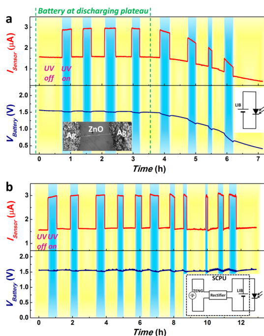
Figure 5. The SCPU as a sustainable power source for driving a UV sensor. (a) Operation of the UV sensor when solely driven by the LIB part in the SCPU, which was recorded from the point that the battery just entered its discharging plateau. The left inset is an optical microscope image of the ZnO-nanowire-based UV sensor in this demonstration, and the right inset is the circuit diagram showing the power source. (b) The operation of the UV sensor continuously driven by the SCPU in the “sustainable mode” for \sim 13 h. The inset is the circuit diagram showing the UV sensor powered by the SCPU in the “sustainable mode”. In both of (a) and (b), the top curve (red) is the current through the sensor, reflecting its response to the UV light, and the bottom curve (blue) is the real time voltage of LIB part.
